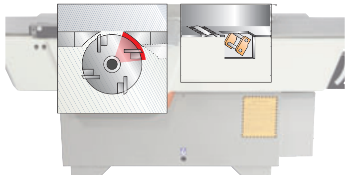
Infeed table moved by parallelogram connecting rods, to adjust stock removal with maximum precision.
