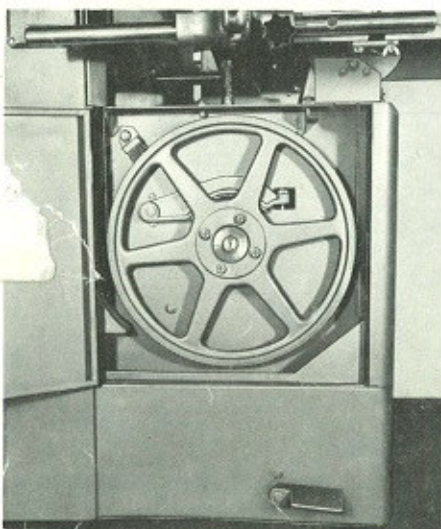
Powerful foot operated brake acts on bottom saw pulley for bringing machine quickly to rest. Brush keeps pulley rim free from dust.
