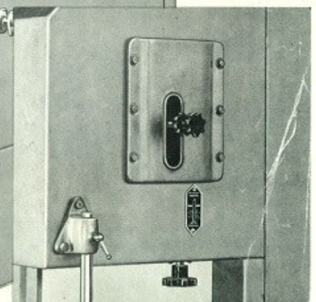
Convenient hand wheel blade tension and tracking adjustments for correct saw setting. Scale indicates tension for varying widths of saws.
